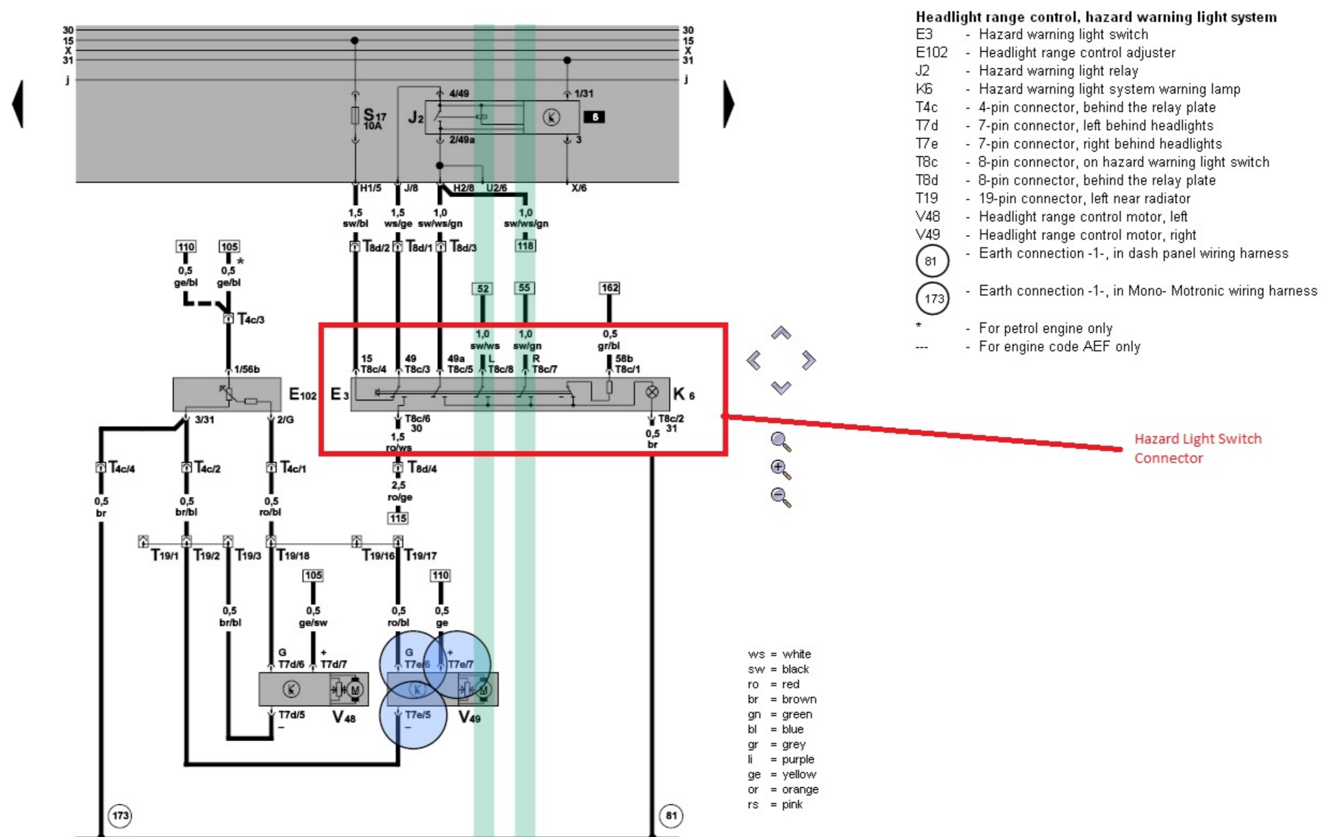
Volkswagen Polo 6n Wiring Diagramgolkes
